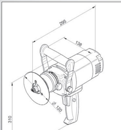
Cutting angle 30°
